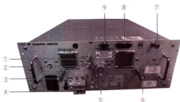
Figure 91 - Interface Description
